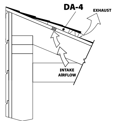
Single-Slope Installation
