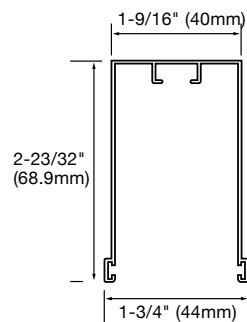
Top Profile
