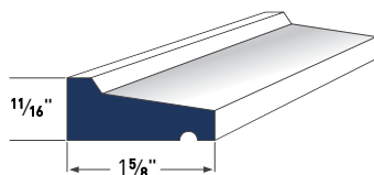
DRIP CAP AZM-197
