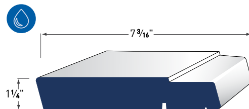
DOUBLE HUNG SILL AZM-7650
