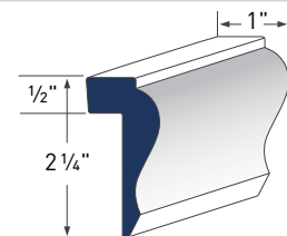
WAINSCOT CAP AZM-284
