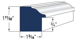
BACK BAND AZM-6931
