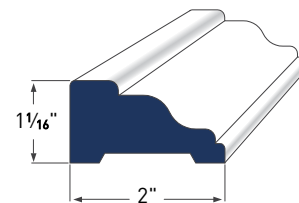
RAKE MOULDING AZM-287
