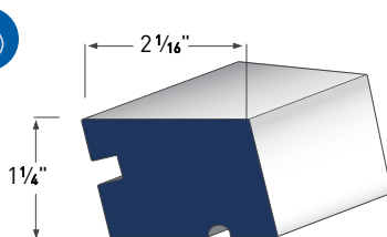
WINDOW SILL NOSE AZM-7974
