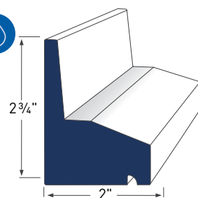
WATER TABLE AZM-6935
