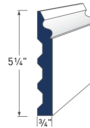
COLONIAL BASE CAP AZM-163
