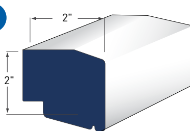
LARGE SILL NOSE AZM-7979
