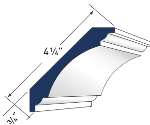
COVE MOULDING AZM-80 LENGTH: 16'
