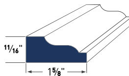
SHINGLE MOULD AZM-210
