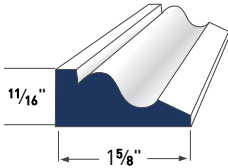
BAND MOULDING AZM-217
